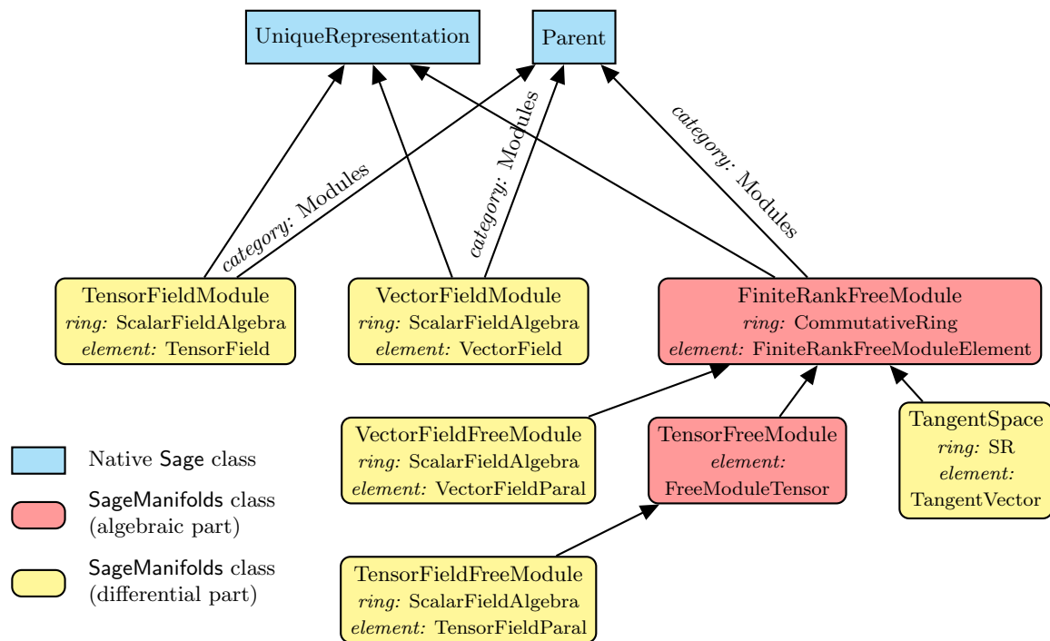
Figure 3. Python classes for modules. For each of them, the class of the base ring is indicated, as well as the class for the elements.
